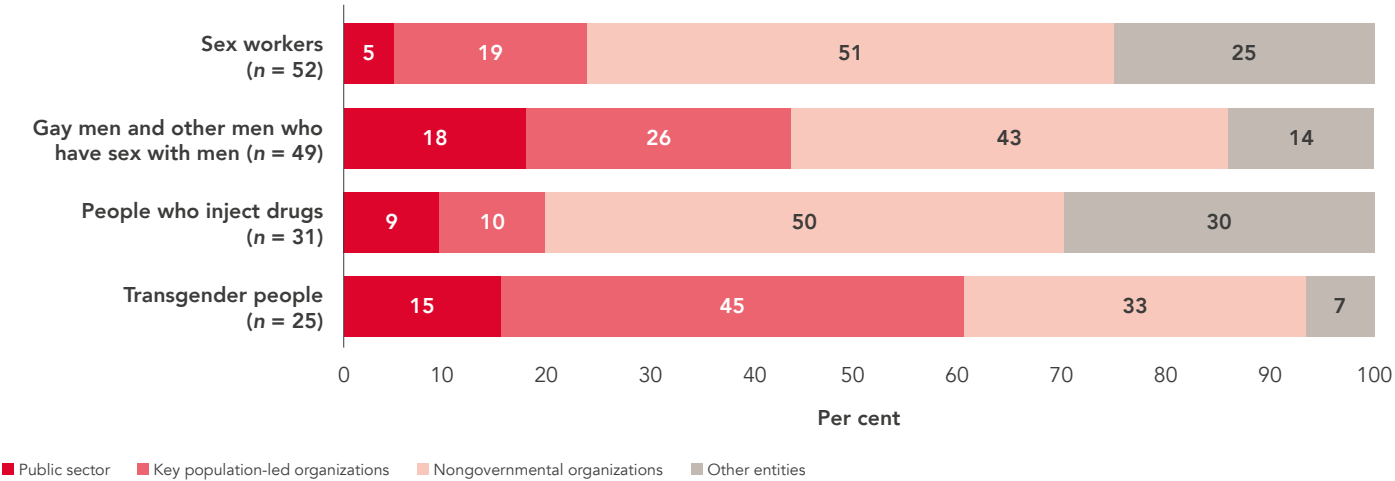
Figure 11 Distribution of the reported numbers of people from key populations reached with HIV prevention interventions, by type of provider, 2020–2024
